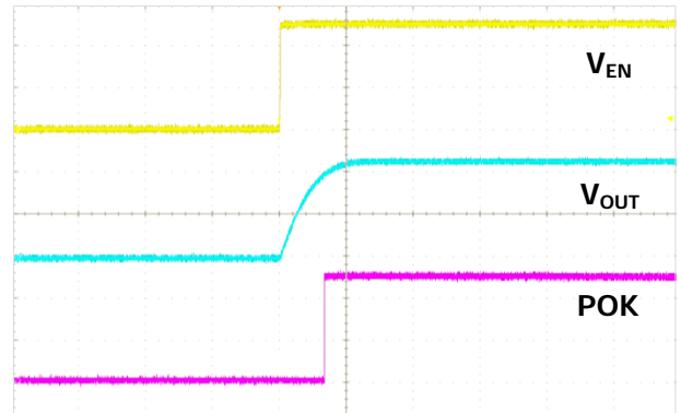
- V_{EN} : 2V/div, V_{OUT} : 500mV/div, POK: 2V/div, 500us/div Start up @ I_{OUT}=2\text{A} , Circuit #1 ( C_{ff}=10\text{nF} , C_{SS}=470\text{pF} , R1=R2=10\text{k}\Omega , V_{IN}=1.7\text{V} , V_{BIAS}=5.0\text{V} )
