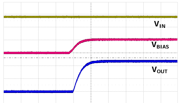
- V_{IN} : 2V/div, V_{BIAS} : 5V/div, V_{OUT} : 500mV/div, 500us/div Start up @ I_{OUT}=2\text{A} , Circuit #2 ( C_{ff}=10\text{nF} , C_{SS}=470\text{pF} , R1=R2=10\text{k}\Omega , V_{IN}=1.7\text{V} , V_{EN}=5.0\text{V} )
