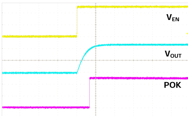
- V_{EN} : 2V/div, V_{OUT} : 500mV/div, POK: 2V/div, 500us/div Start up @ I_{OUT}=10\text{mA} , Circuit #1 ( C_{ff}=10\text{nF} , C_{SS}=470\text{pF} , R1=R2=10\text{k}\Omega , V_{IN}=1.7\text{V} , V_{BIAS}=5.0\text{V} )
