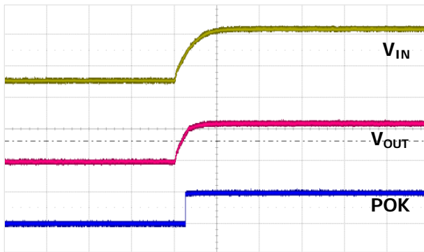
- V_{IN} : 1V/div, V_{OUT} : 1V/div, POK: 5V/div, 500us/div Start up @ I_{OUT}=10\text{mA} , Circuit #1 ( C_{ff}=10\text{nF} , C_{SS}=470\text{pF} , R1=R2=10\text{k}\Omega , V_{EN}=V_{BIAS}=5.0\text{V} )
